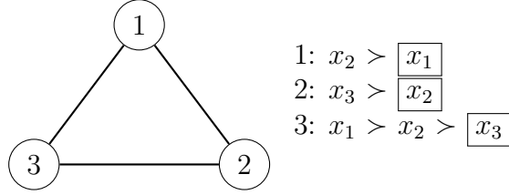
Figure 1.1: Example for REACHABLE ASSIGNMENT on a cycle with n = 3 and preference lists on the right hand side. For the sake of simplicity, the target assignment \sigma is simply the most preferred object of each agent. The object inside the box is the object that the corresponding agent initially holds. An exemplary sequence of swaps such that every agent reaches its most preferred object is the following. First, agent 2 and 3 swap their currently held objects. Agent 2 then owns object x_3 , which it prefers the most and agent 3 owns object x_2 . Afterwards, agent 1 can trade object x_1 to agent 3 and receive object x_2 in return. Every agent then owns its most preferred object.
