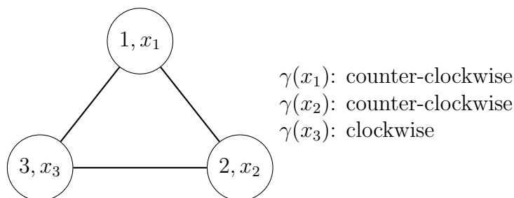
Figure 4.1: Example for two objects in swap position. We assume that none of the three objects has reached its destination. Object x_3 is assigned clockwise direction and will therefore pass agent 1 next on its path. Object x_1 is assigned counter-clockwise direction and will therefore pass agent 3 next. The objects x_3 and x_1 are therefore in swap position. Agent 2 is also a neighbor of agent 3. Further the object assigned to agent 2, namely x_2 , and the object assigned to agent 3, namely x_3 , are also assigned opposite direction. However, the two objects are not facing each other and are therefore not in swap position.
